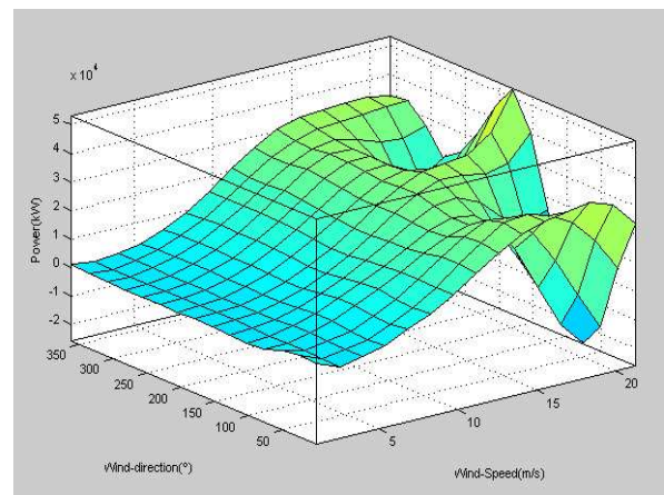
Figure 5: A two-dimensional power curve model
